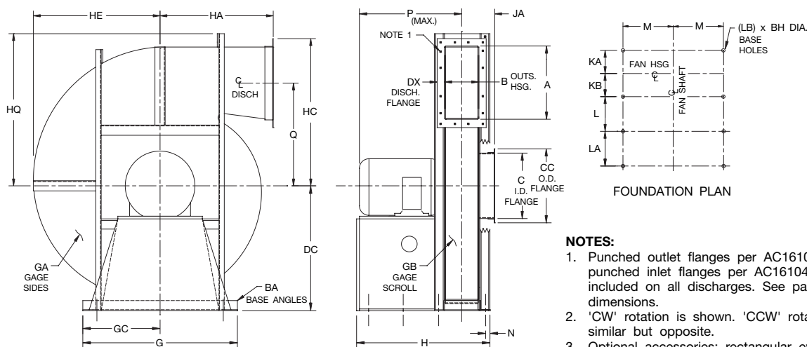
CLOCKWISE ROTATION, TOP HORIZONTAL DISCHARGE 'CW THD'
