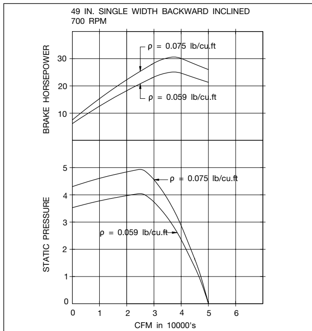
Figure 3. Test Points at Different Air Densities
