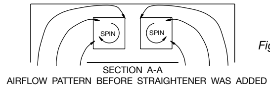
Figure 18. Duct System
