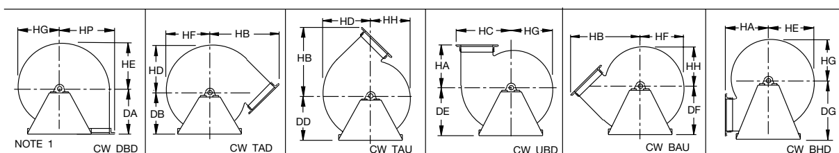
WITH OPTIONAL FLANGED INLET
