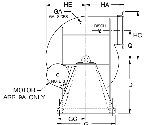
CW THD NON-ROTATABLE
