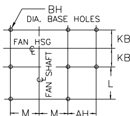
FOUNDATION PLAN
