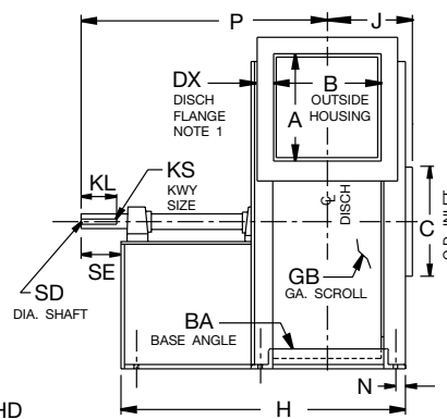
CW THD NON-ROTATABLE
