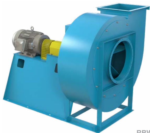
RBW Arrangement 8
