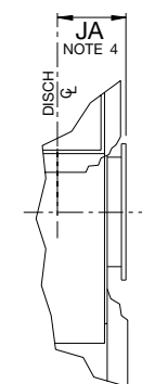
WITH OPTIONAL FLANGED INLET
